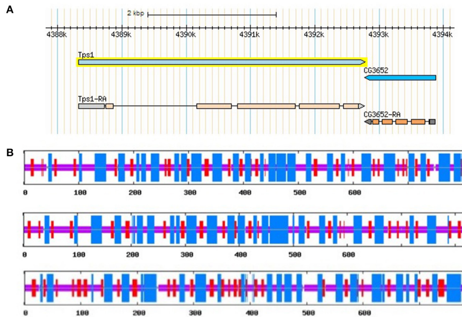
FIGURE 3 | D. melanogaster TPS genomic structure (A) from FlyBase and predicted secondary structures of three TPS proteins of the brown planthopper, including TPS1, TPS2, and TPS3 (B). Blue and red regions represent \alpha -helices and \beta -sheets in Figure 3B, respectively.
